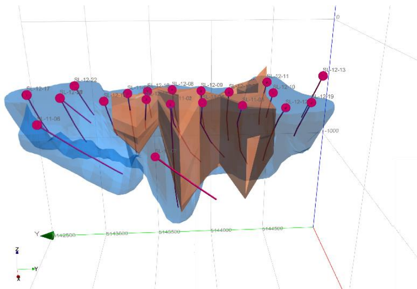
Figure 1. Springer REE Deposit (blue), with Gallium (brown) Core.
